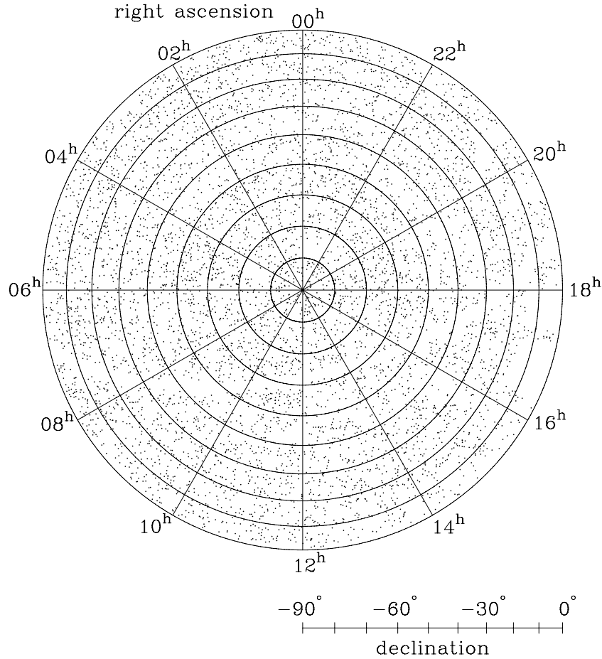
Figure 8. A plot in the equal-area Lambert projection showing the distribution of the 5890 sources in the AT20G catalogue. Note that the catalogue excludes the Galactic plane ( b < 1.5^\circ ) and that some regions north of \delta = -15^\circ are incomplete due to bad weather.
