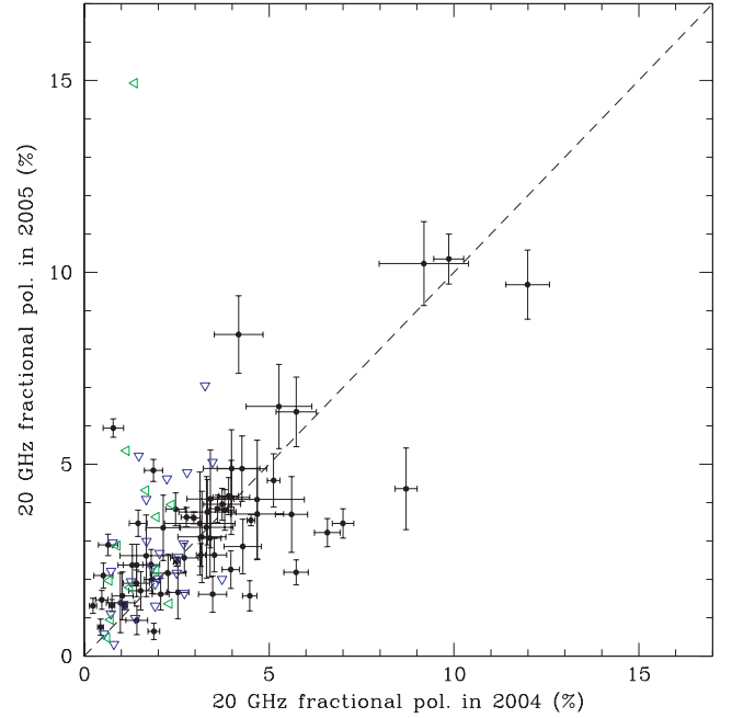
Figure 11. Comparison of fractional polarization at 20 GHz measured in our 2004 October and 2005 October observing runs. Crosses show measured polarization values, and triangles show limits in one of the epochs.
